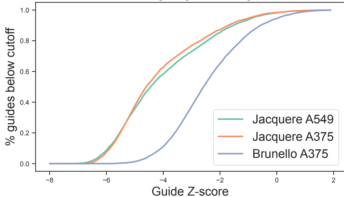
Guides targeting essential genes
