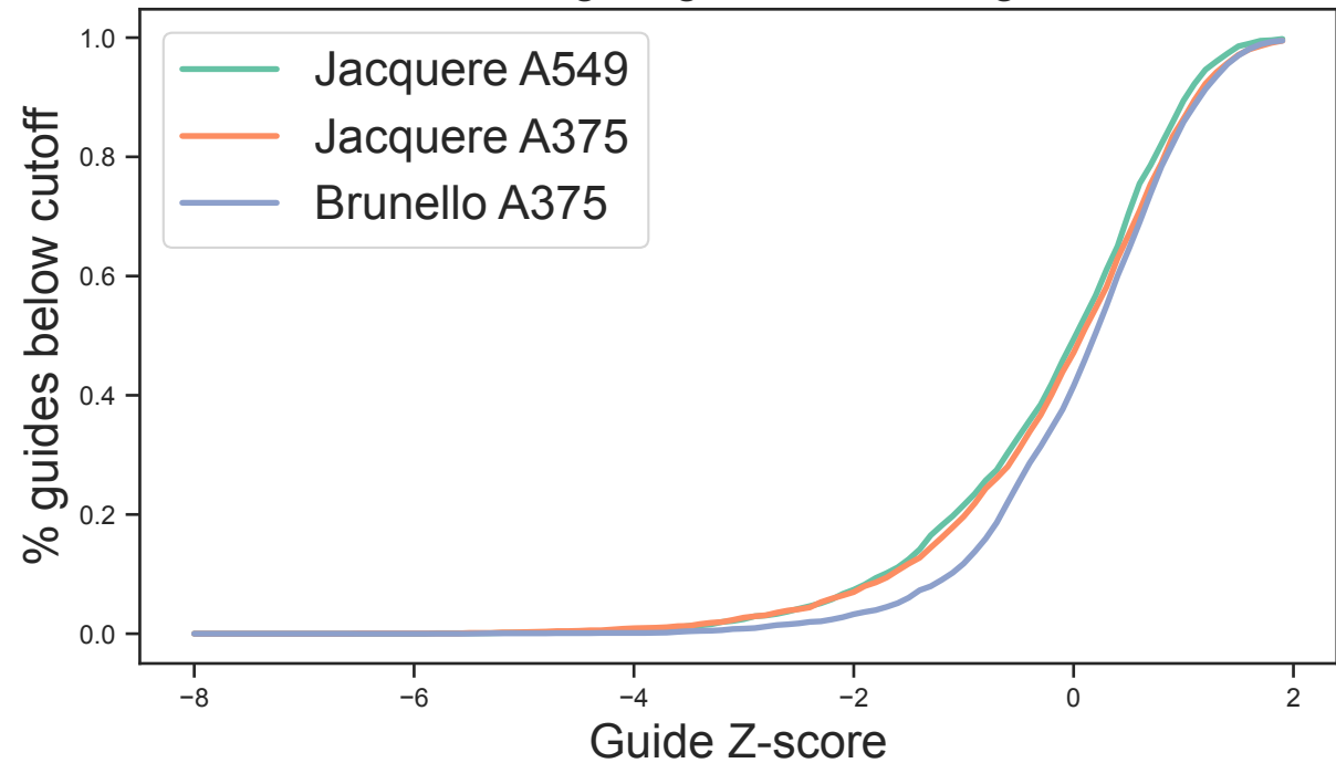
Guides targeting nonessential genes
